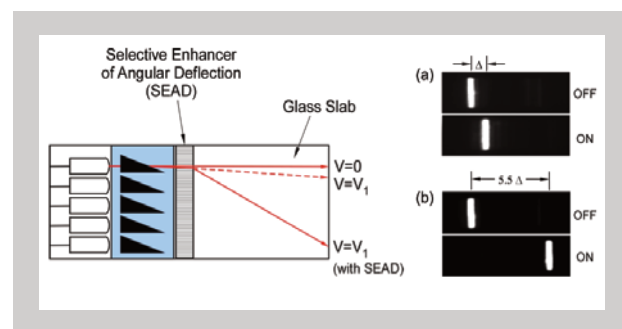
Angular magnification with BragGrate™ Deflector in electro-optic switches.
