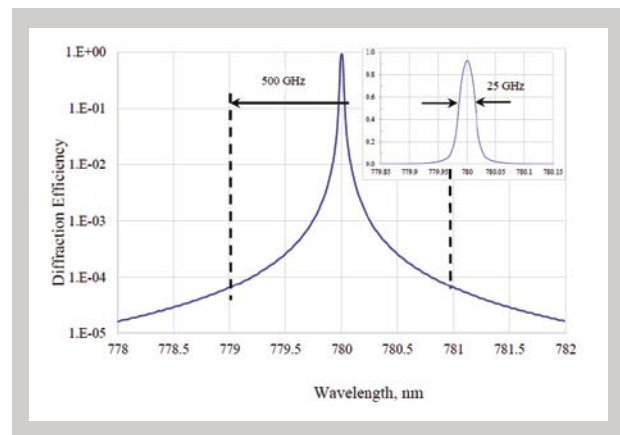
Spectral shape of Filters with Bandwidth 25 GHz
