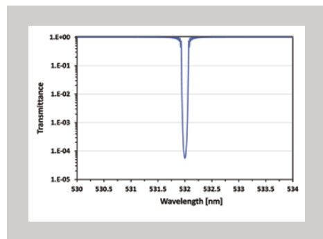
Transmission spectrum of OD4@532 nm BragGrate™ Notch Filter
