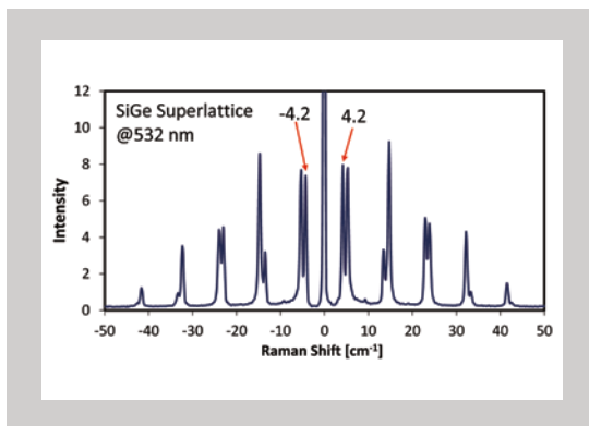
Ultra-low frequency Raman spectrum of SiGe superlattice at 532 nm with LabRAM HR Evolution and BragGrate Notch Filters (Courtesy of HORIBA Jobin Yvon)
