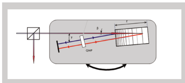
Schematic Diagram of CBG deployment for Qubit Filtering and Control
