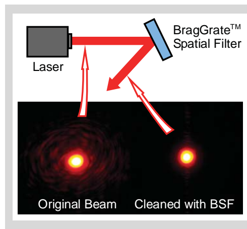
Spatial filtering of 632.8 nm HeNe laser with BSF
